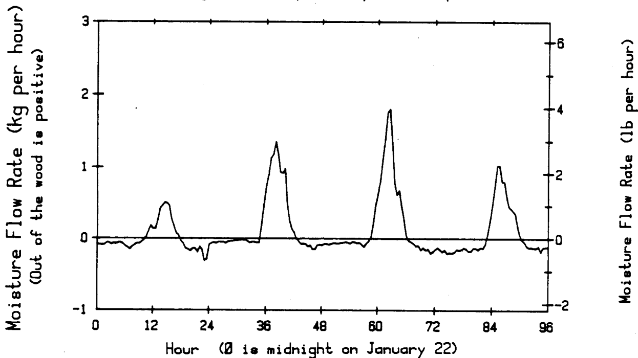
Figure 4. Moisture flows into and out of the wood members of the Oroville attic, January 22 to 25, 1984
