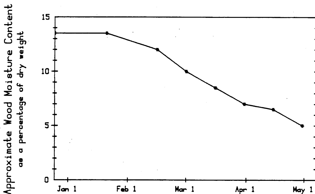
Figure 6. Percentage wood moisture content (kg of water per 100 kg of dry wood) for the Oroville attic for the winter 1983-1984
