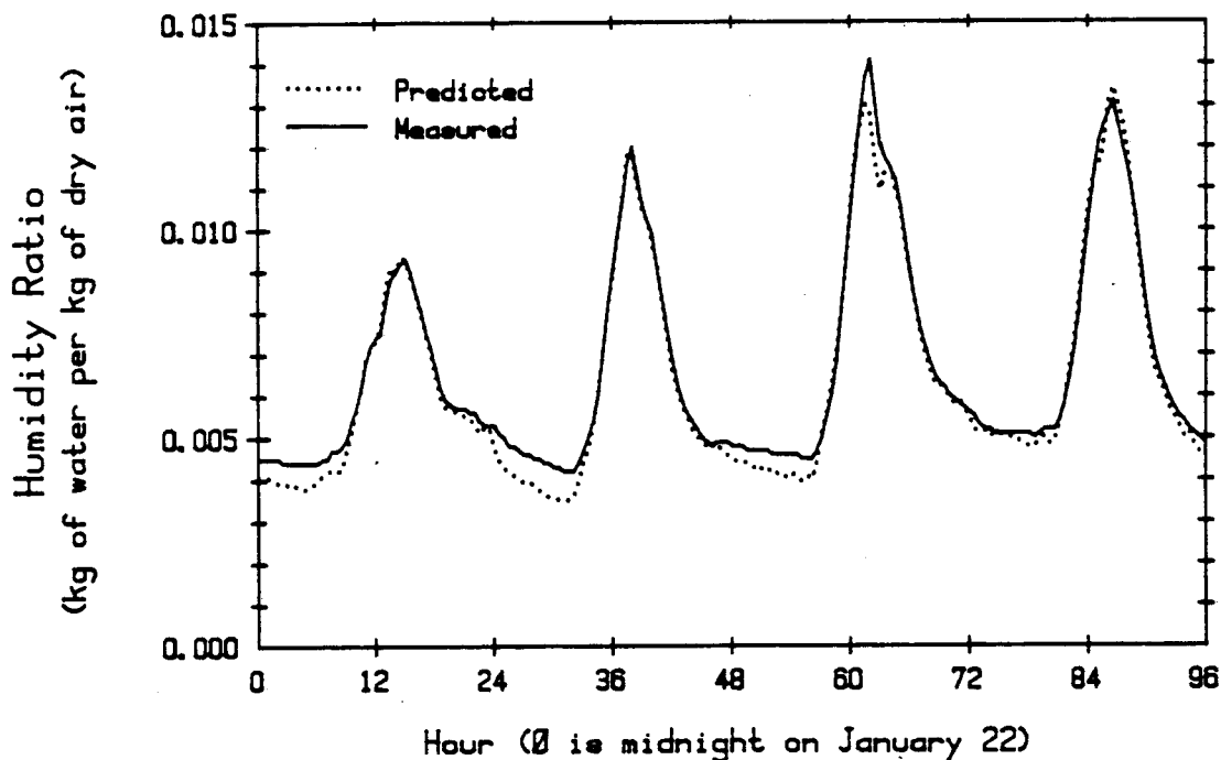
Figure 5. Measured attic air humidity ratio compared with that predicted from Equation 4. Data is for the Oroville attic for the period January 22 to 25, 1984.
