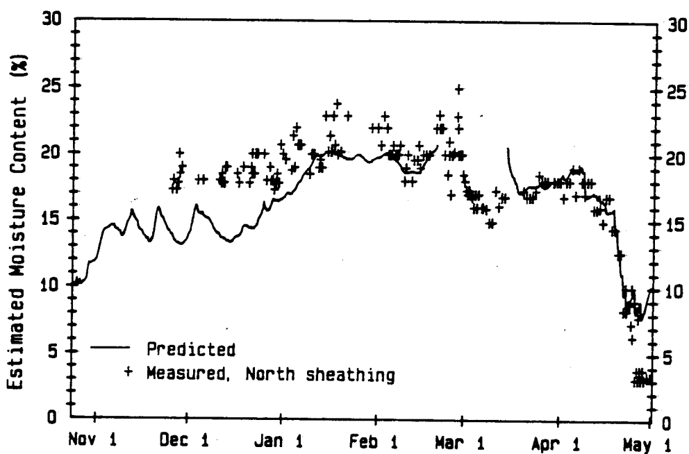
Figure 7. Measured wood moisture content (kg of water per 100 kg of dry wood) compared with that predicted by theory for the winter of 1982-83 for an attic in Madison, Wisconsin.
