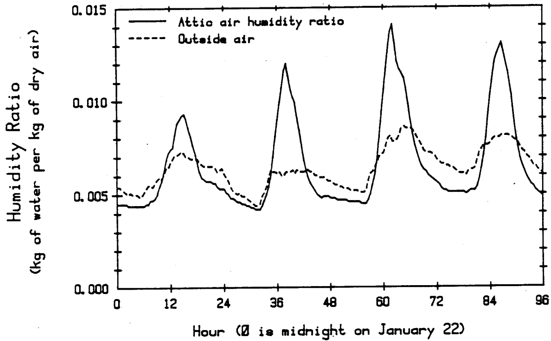
Figure 2. Humidity ratio of the outside air and of the air inside the attic of the Oroville house, January 22 to 25, 1984
