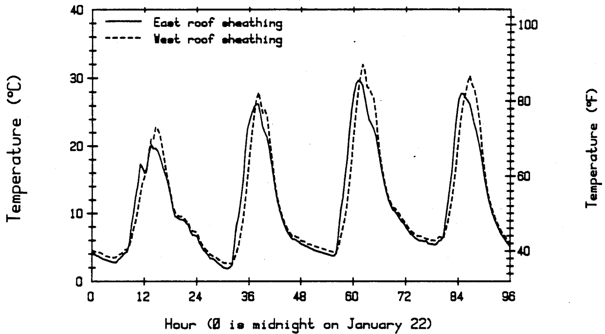
Figure 3. Temperatures of the underside of the roof sheathing in the attic of the Oroville house, January 22 to 25, 1984
